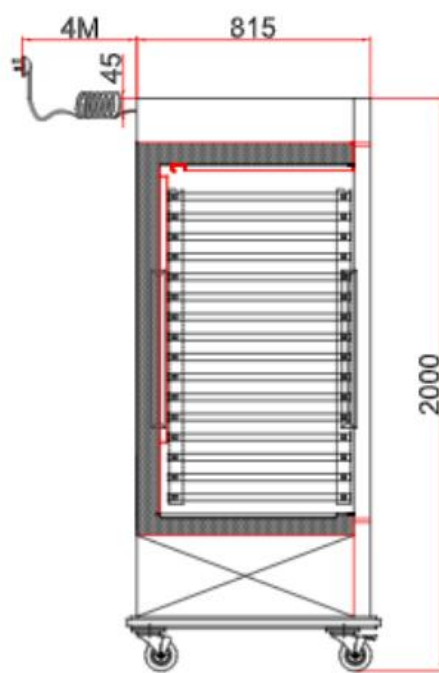
SIDE VIEW 左侧视图
