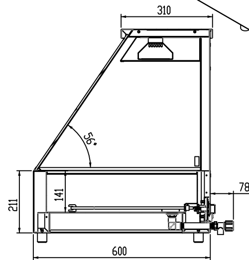
SECTION CF-CF
